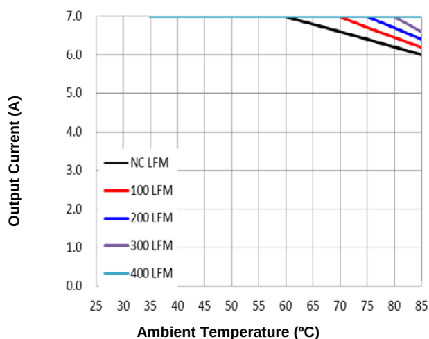
Figure 7. Current Derating Curve for Airflow Direction 3 (Ref. Fig. 8 for Airflow Direction; typical Vin, open frame, soldered interface)
